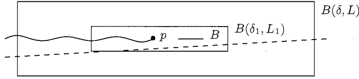
FIGURE 2. The time the ellipse (drawn here as a dashed line) spends inside the small box B(\delta_1, L_1) is at most \epsilon times the time the ellipse spends in the larger box B(\delta, L) . In Lemma 7.10, this is proved as a result in (\mathbb{R}^2)^k . Because of Lemma 7.12, it can be transferred to \mathcal{X}^k , even if the ellipse crosses the branch cut starting at the possibly singular point p .
